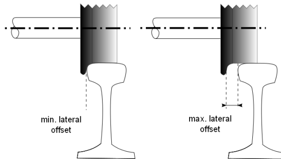
Figure 1: Lateral offset principle
